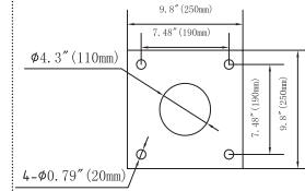
Anchor Bolt Positioning Plate
