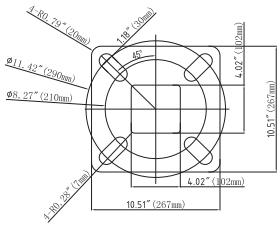
4" Flange
