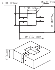
Flange Base Cover
