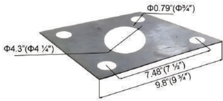
Screw Positioning Plate
