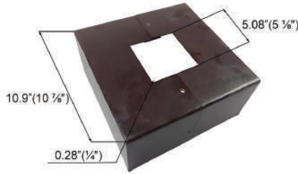
Base Shield
