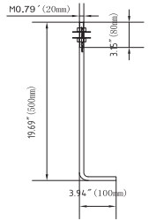
Anchor Bolt
