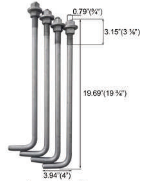
Anchor Bolts
