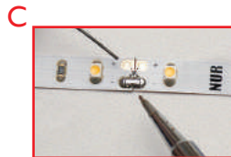
C: Two terminated ends can be soldered to one another.
