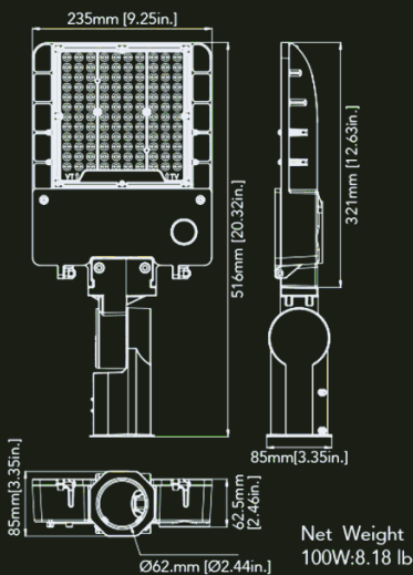
Slipfitter Mount (100W)
