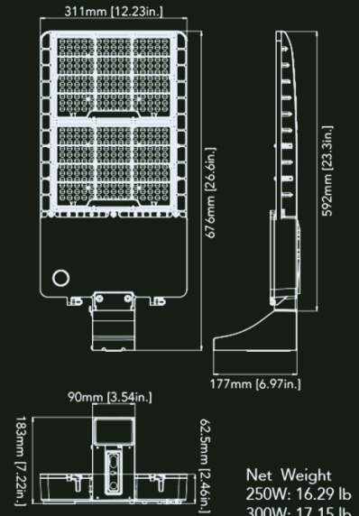
Pole Mount (250W&300W)
