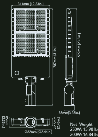
Slipfitter Mount (250W&300W)
