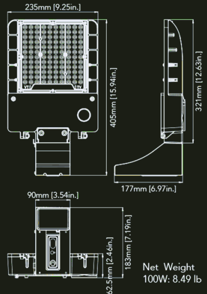
Pole Mount (100W)
