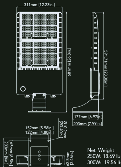
Wall Mount (250W&300W)
