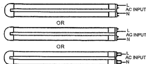
Double Ended Input
