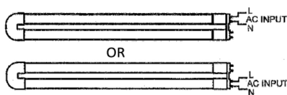
Single Ended Input
